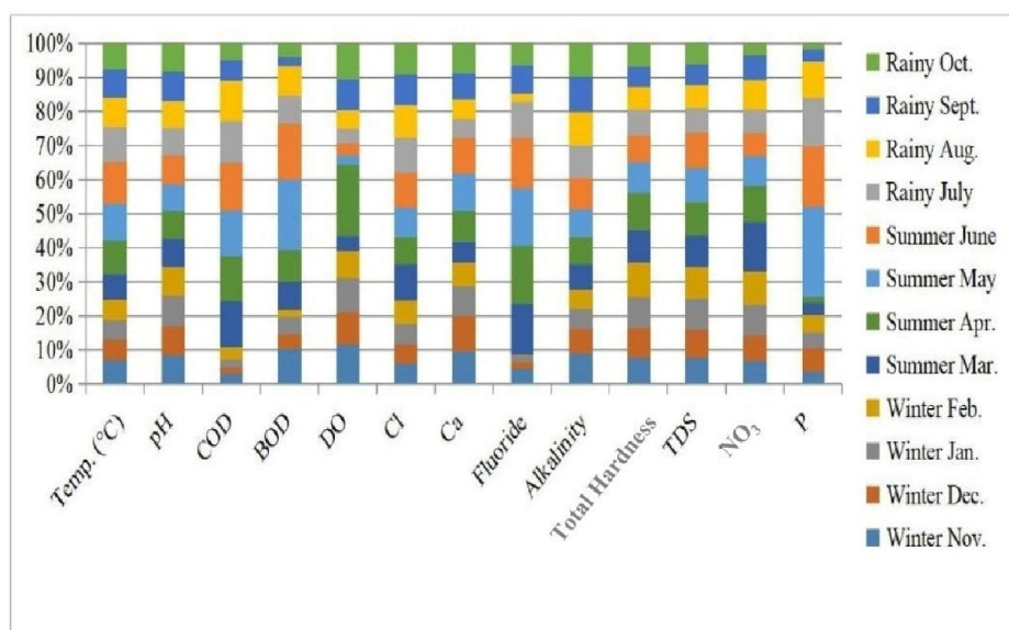
Figure 1. Monthly, seasonal and annual variation of physicochemical parameters in Jangali Pond (November, 2014 to October, 2015).
