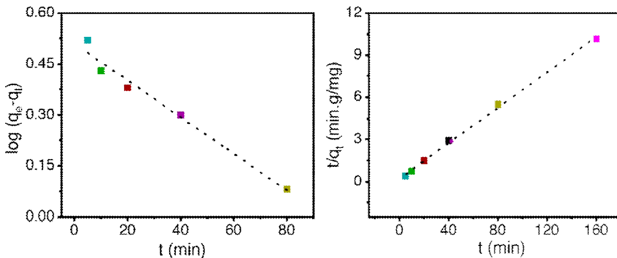
Figure 4. Shows the (A) pseudo-first-order kinetics plot and (B) pseudo-second-order kinetics plot.
